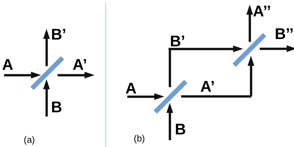
Figure 1: Depiction of a beam splitter
